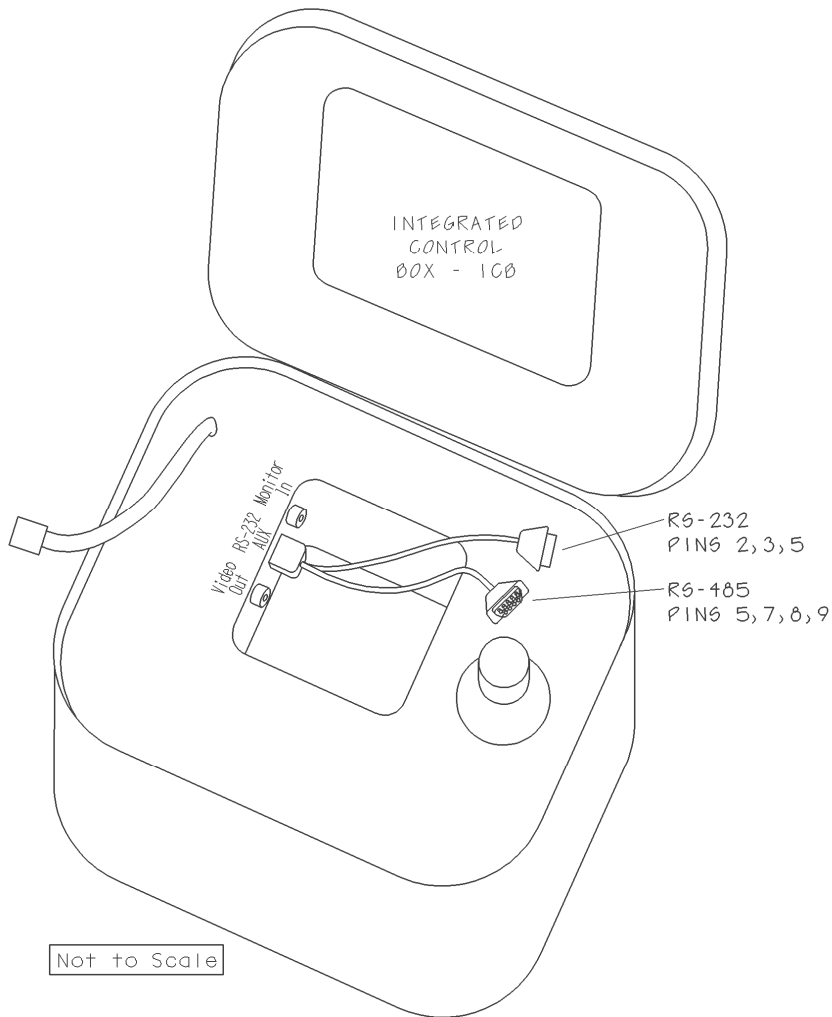
Figure 4 – Accessory Splitter connected to Integrated Control Box
